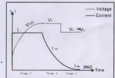
Charging Curve
